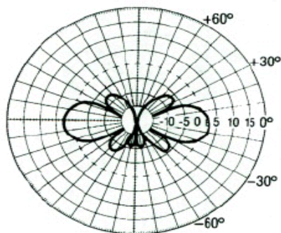
Diagrama de Radiación Vertical Vertical Radiation Pattern
